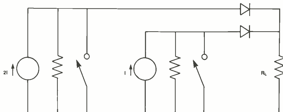
Figure 1. A 2-switch modulator illustrates the concept of digital modulation. The current sources are binarily related, and between them provide four output states.
